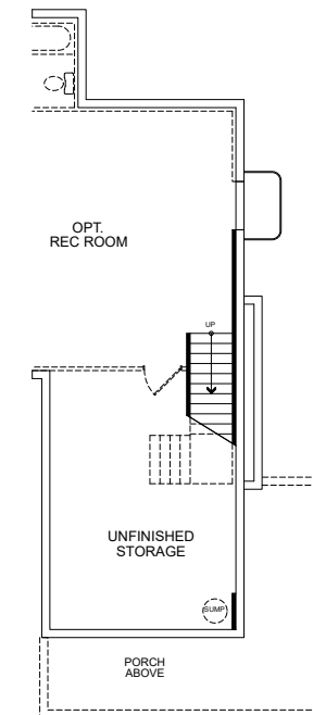
OPTIONAL ENHANCED SIDE W/ WRAPPED PORCH BASEMENT
