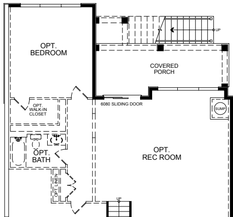
Optional Walk-Out Basement
