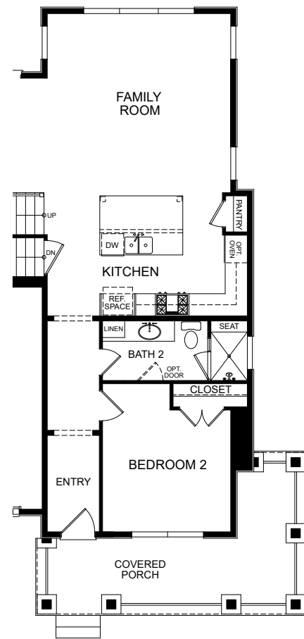
OPTIONAL ENHANCED SIDE W/ WRAPPED PORCH MAIN LEVEL
