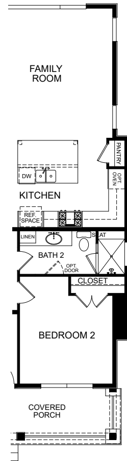
OPTIONAL ENHANCED SIDE MAIN LEVEL
