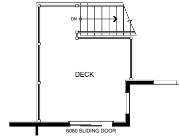
OPTIONAL WALK-OUT DECK
