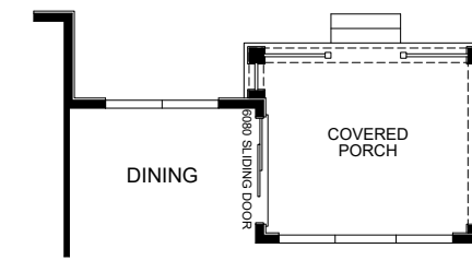
OPTIONAL REAR COVERED PORCH
