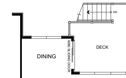
OPTIONAL WALK-OUT DECK
